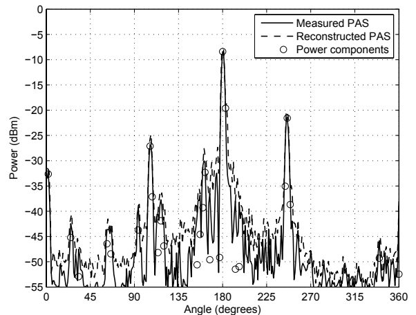
Figure 7: Received and reconstructed PAS for office environment, Location 1
