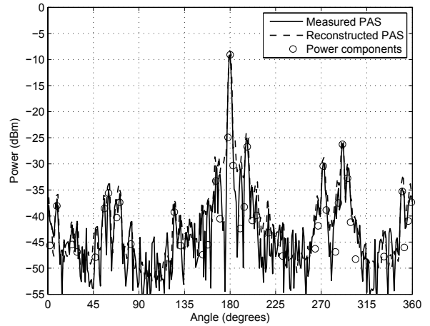
Figure 5: Received and reconstructed PAS for home environment, Location 1
