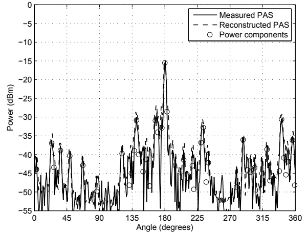
Figure 6: Received and reconstructed PAS for home environment, Location 2
