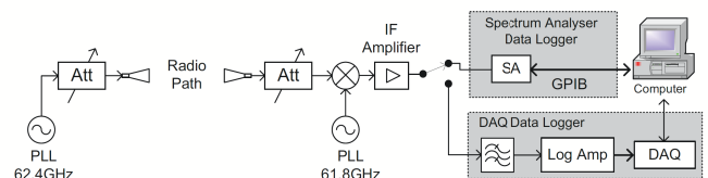
Figure 1: Measurement system
